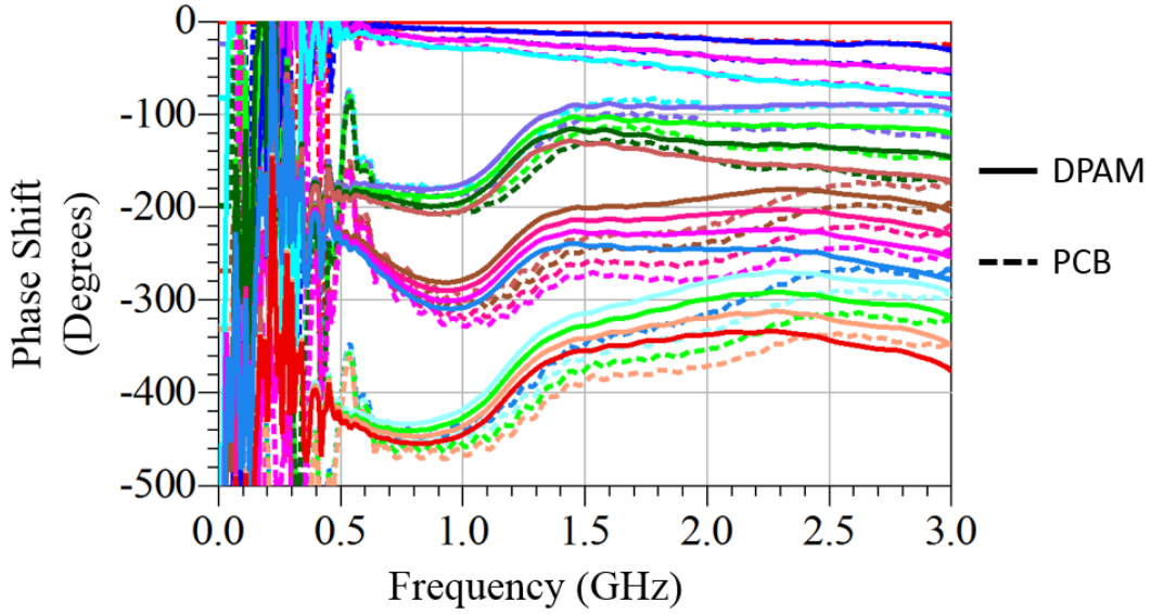
Figure 3.9- Measured relative phase shift of DDM and PCB 4-bit phase shifters
