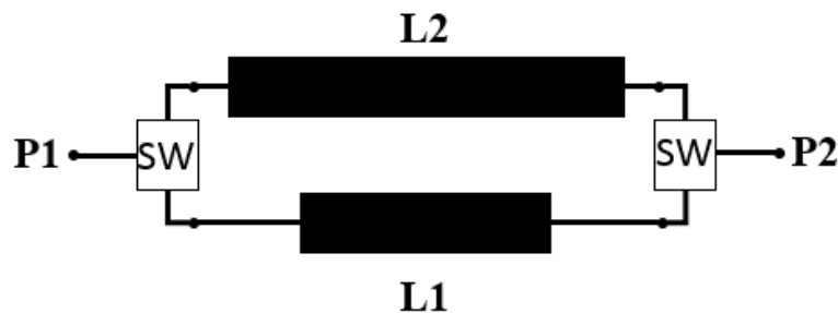
Figure 2.4- Switched line (delay line) phase shifter topology
